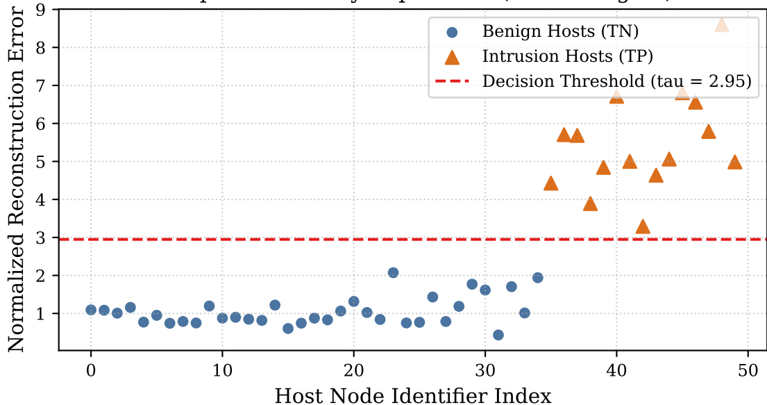
Temporal Anomaly Separation ( k = 2.5 sigma)
