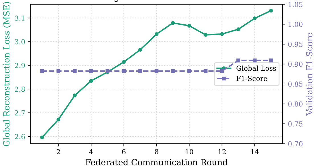
Fed-GNIDS Convergence Across Communication Rounds
