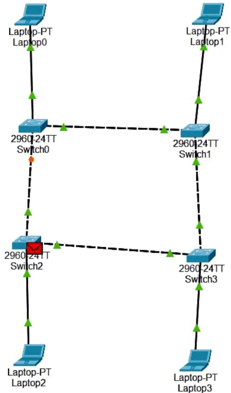
Dillip A Ring topology
