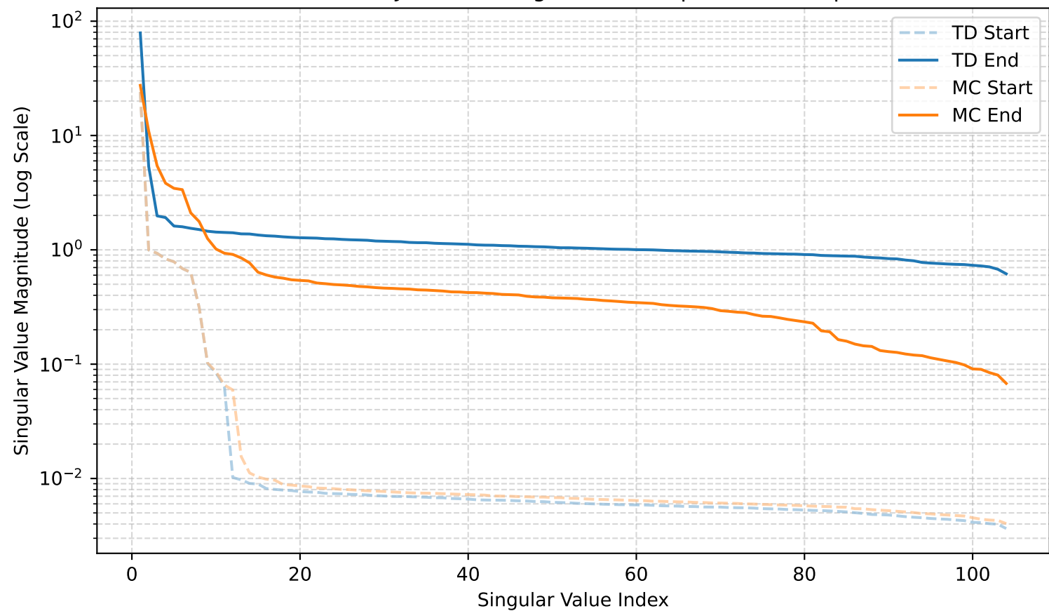
Environment - Jacobian Singular Value Spectrum Comparison
