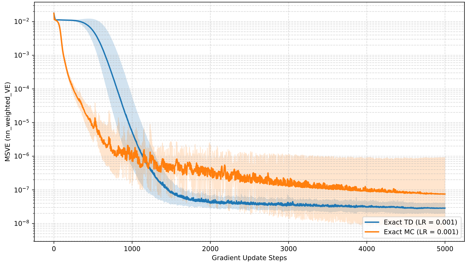
Value Error Comparison over Training Course
