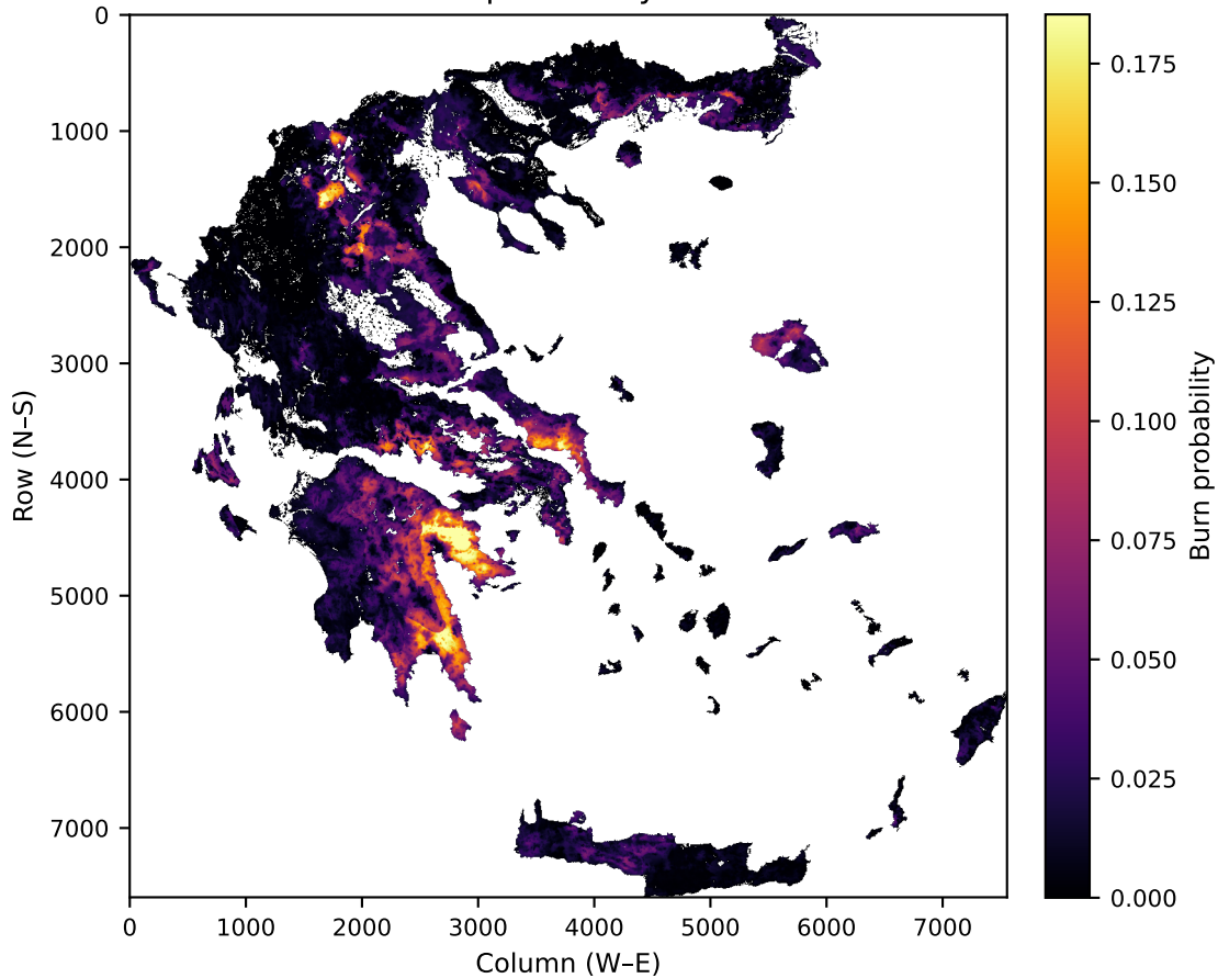
FSim burn probability — Greece
