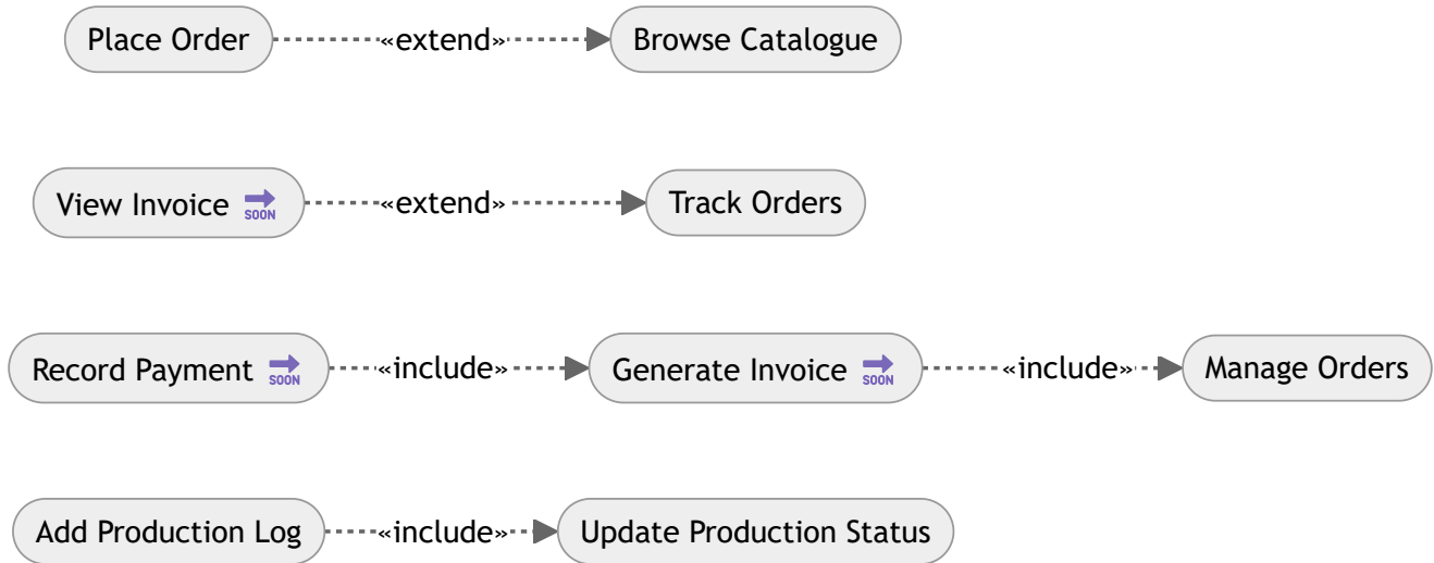
Figure 4 — Include & Extend Relationships
