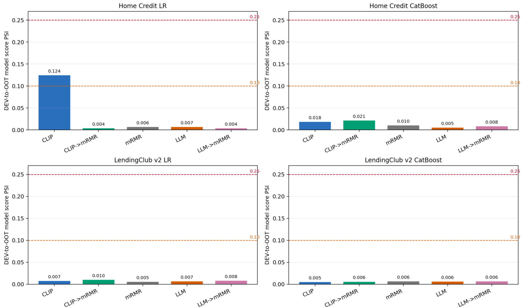
Figure 3. DEV-to-OOT model score PSI comparison
