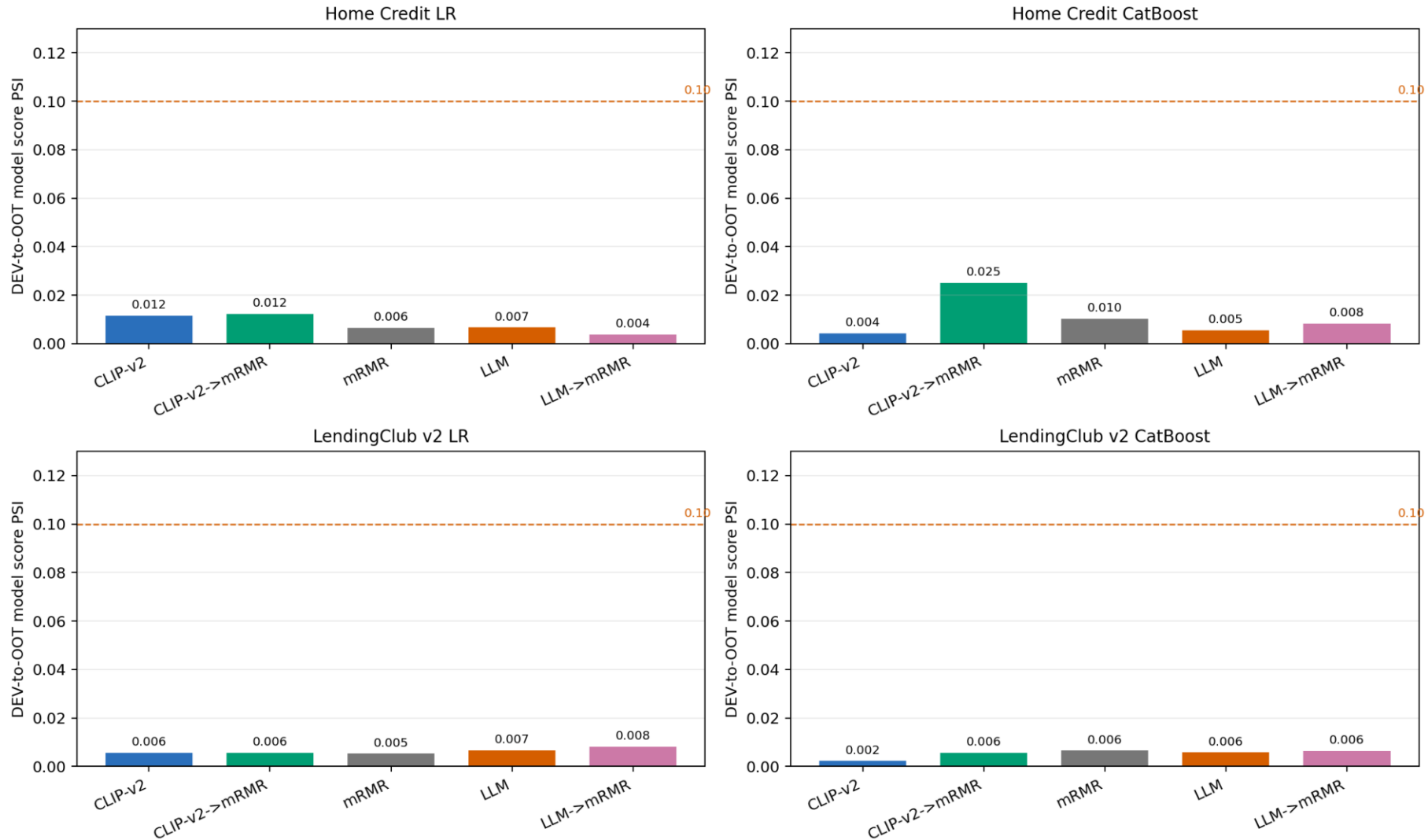
Figure 3. CLIP-v2 DEV-to-OOT model score PSI comparison
