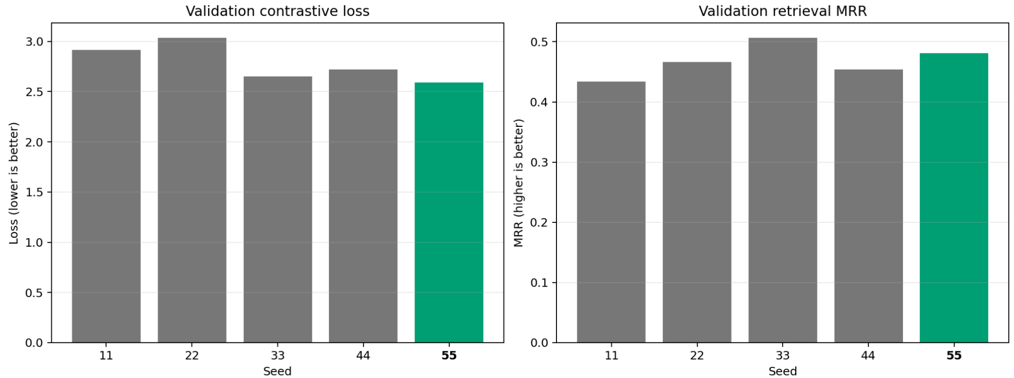
Figure 5. CLIP seed robustness (selected seed 55)
