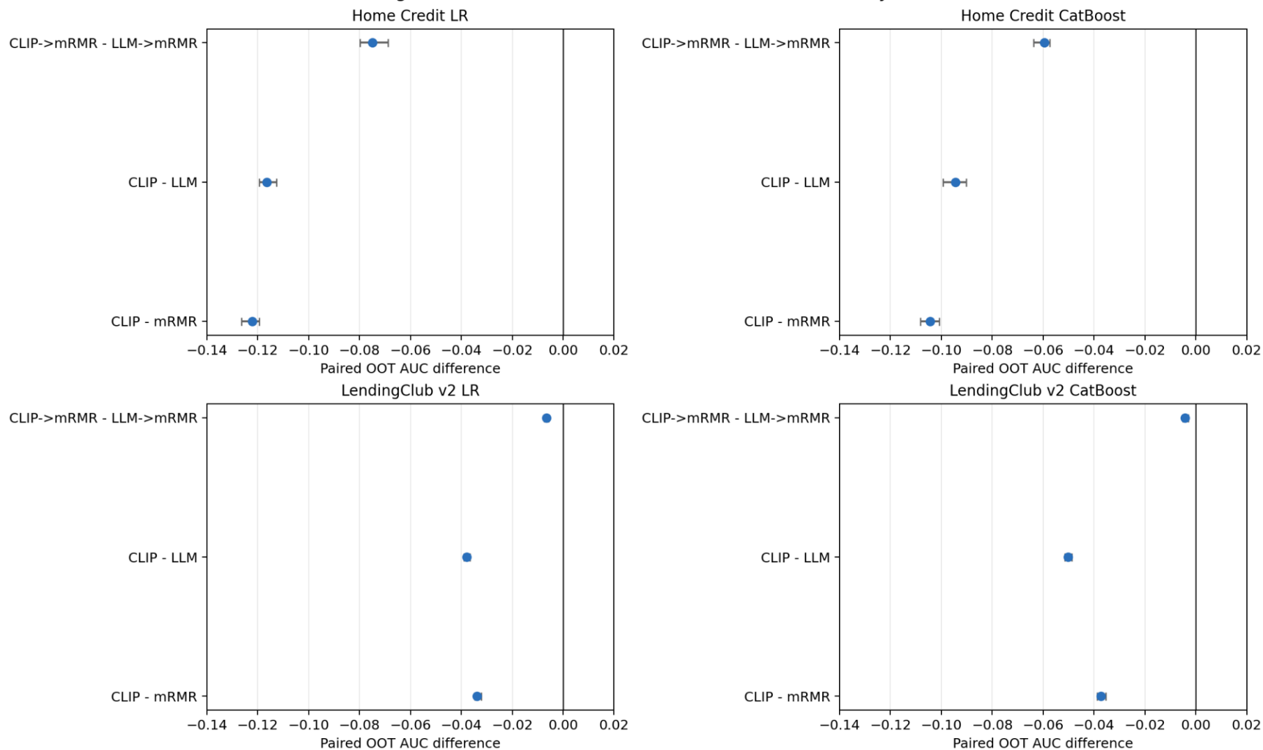
Figure 2. Paired OOT AUC differences with uncertainty
