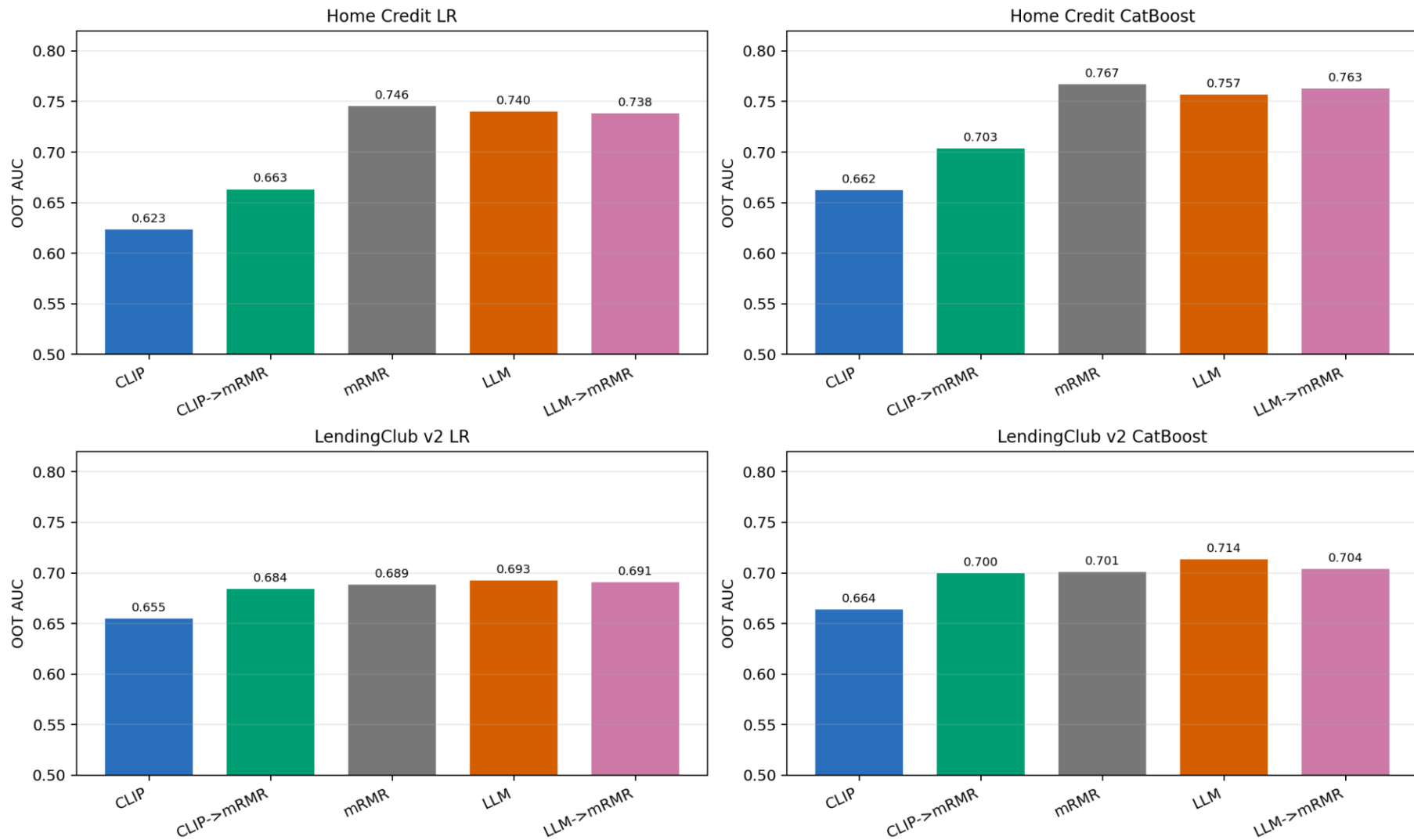
Figure 1. Main OOT AUC comparison
