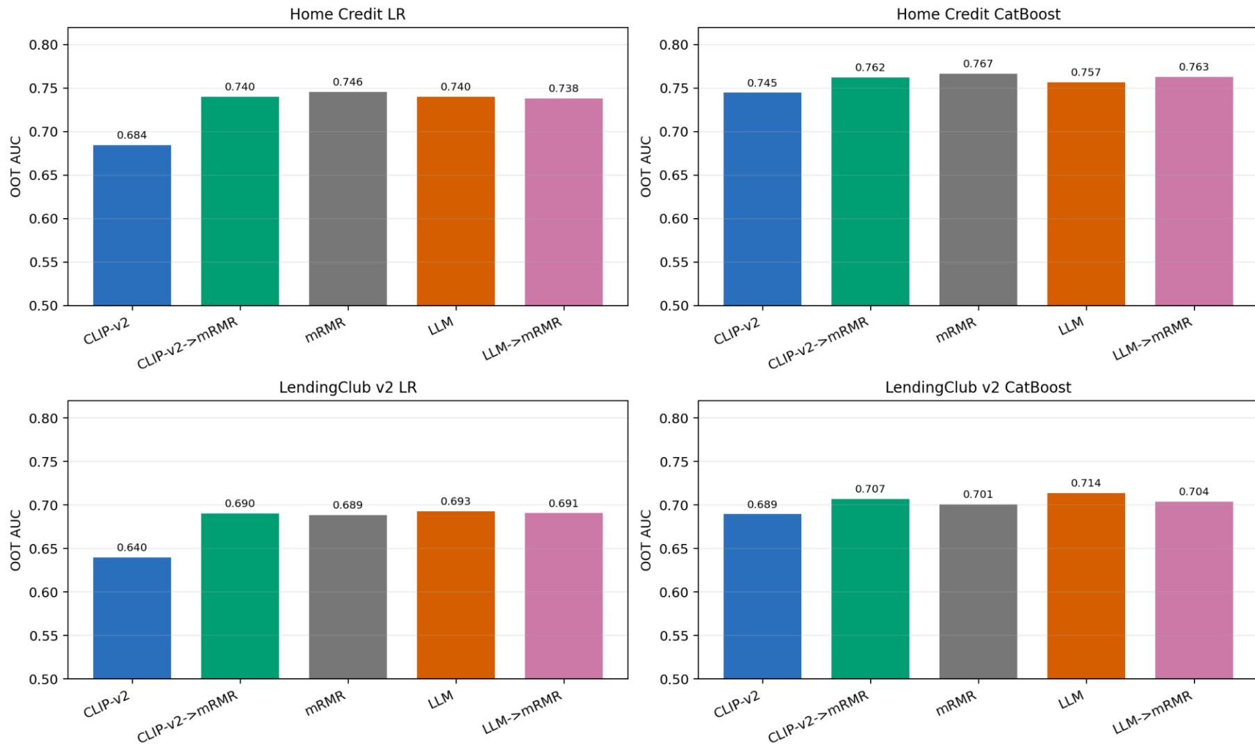
Figure 1. CLIP-v2 OOT AUC comparison
