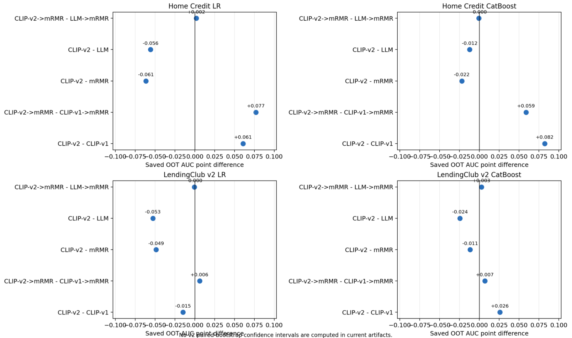
Figure 2. CLIP-v2 OOT AUC deltas
