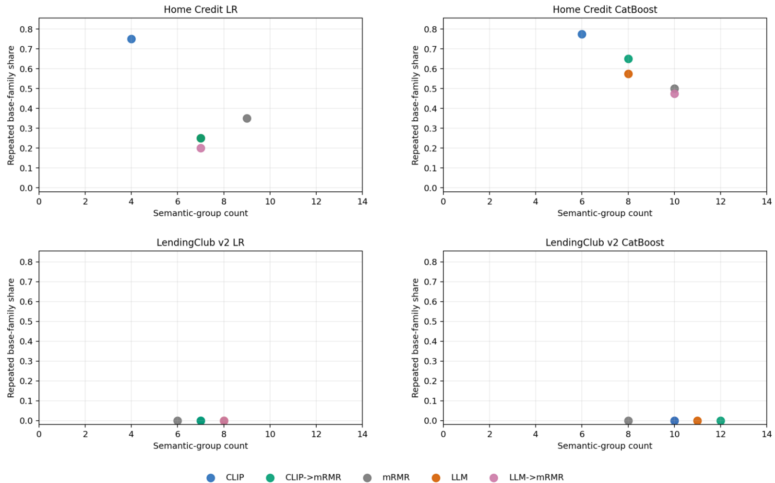
Figure 4. Semantic coverage and redundancy
