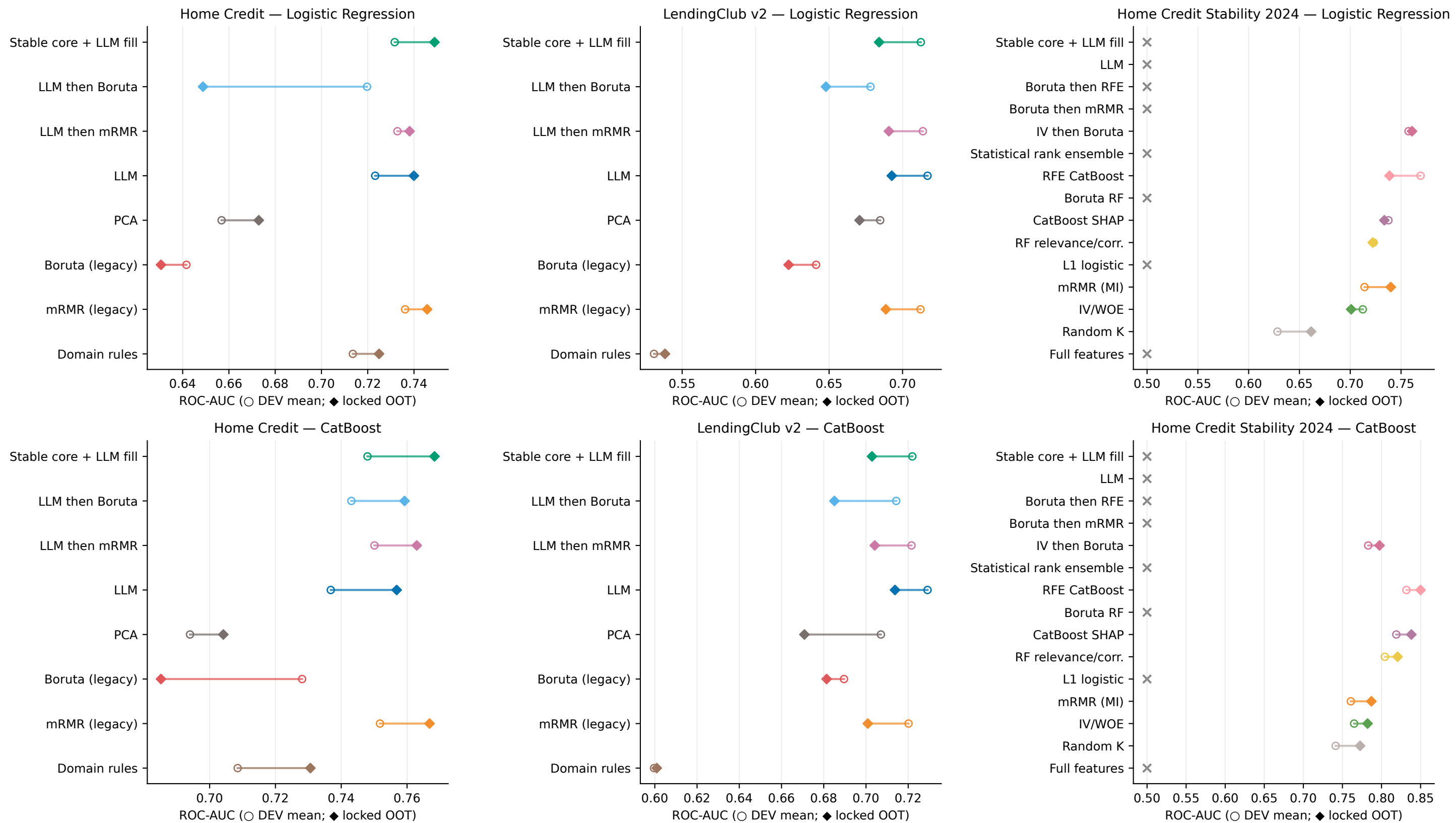
Figure 2. DEV-to-OOT performance dumbbells
