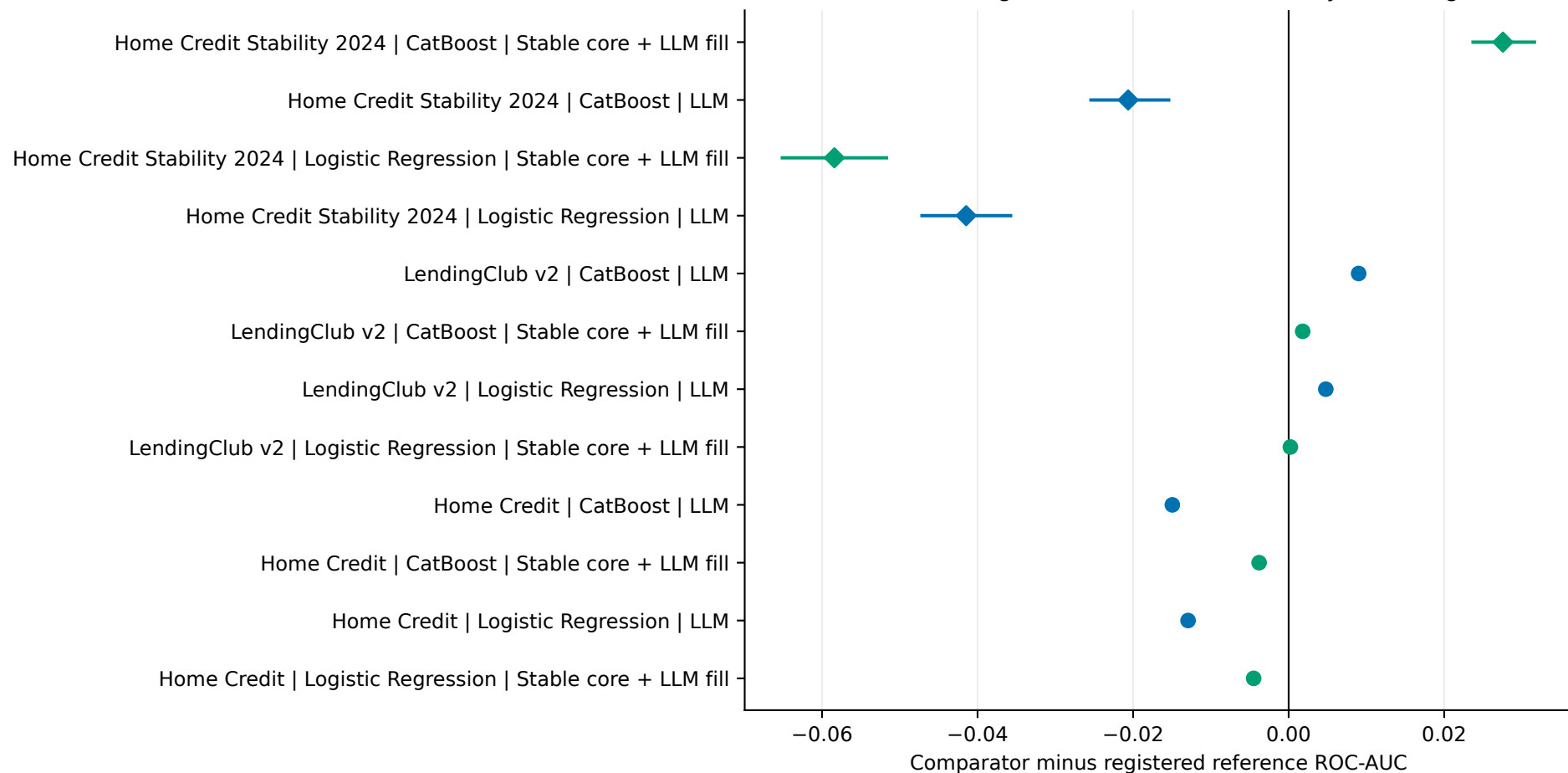
Figure 5. LLM-assisted versus matching classical effects Diamond = Holm-significant; intervals shown only where registered
