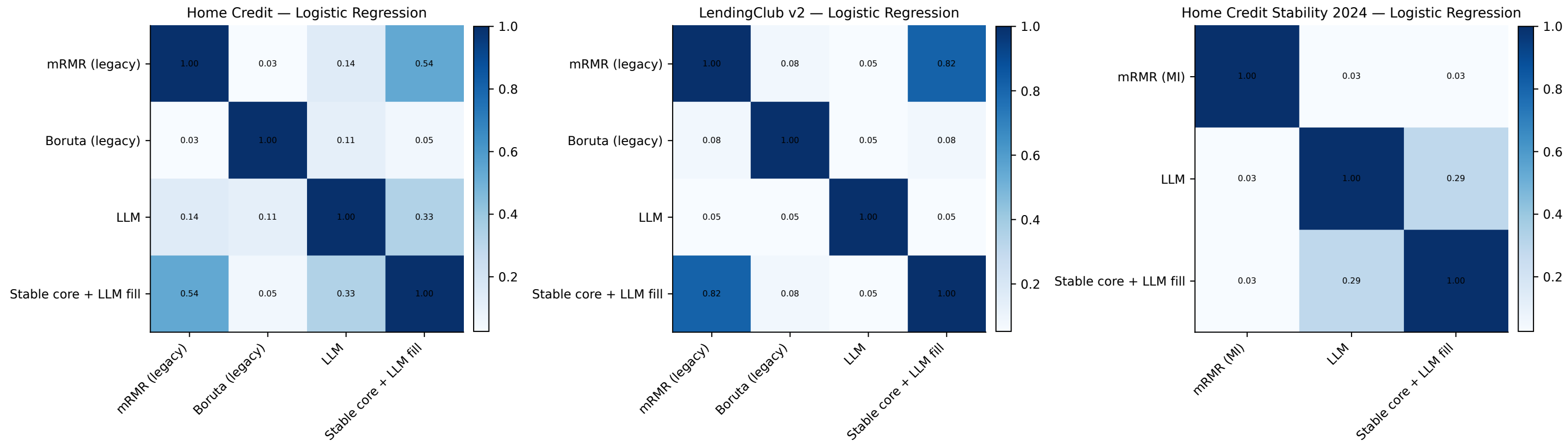
Figure 10. Within-dataset final-selection overlap (Jaccard)
