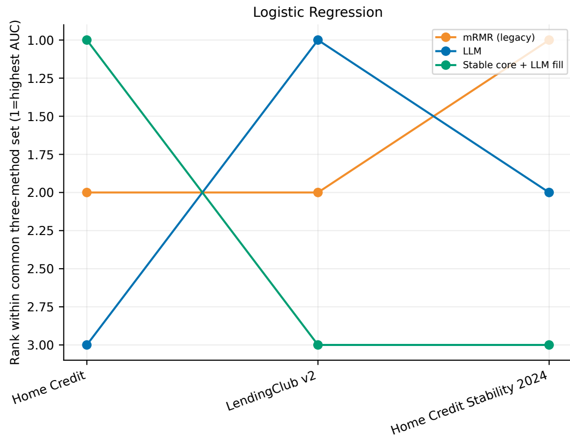
Figure 14. Cross-dataset rank consistency on a common method set
