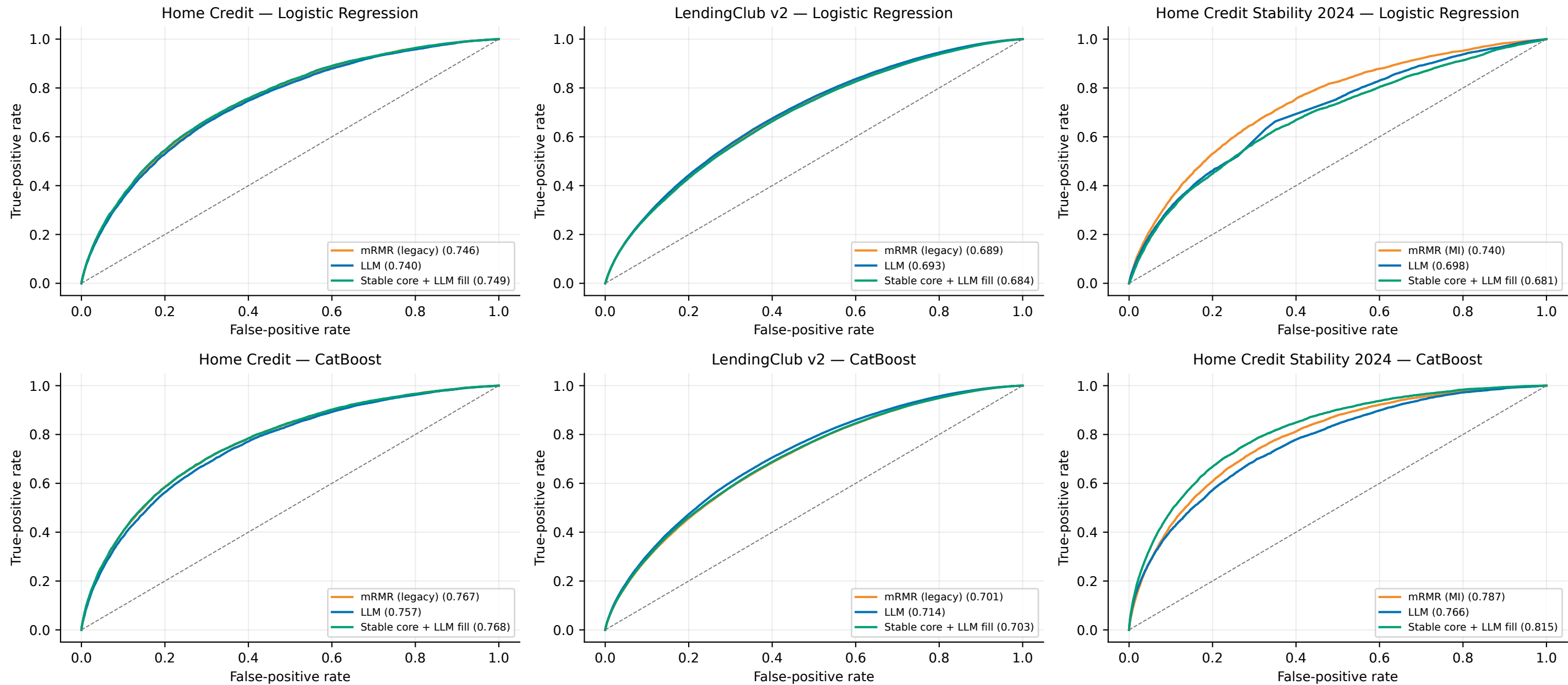
Figure 15. Protocol-fixed subset of locked OOT ROC curves
