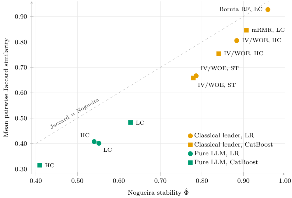
Figure 3: Reproducibility landscape of fold-level selections. Orange: most reproducible refitted classical selector in each dataset–backbone case; green: pure LLM lists cached per fold on Home Credit and LendingClub. Circles are logistic regression ( K = 20 ), squares CatBoost ( K = 40 ). HC = Home Credit, LC = LendingClub v2, ST = Stability 2024. Higher is more reproducible on both axes; the dashed line marks equality of the two statistics. The Nogueira universe is the screened candidate set of the dataset for every point shown, so all points are on a common scale within a dataset; because the chance correction depends on d , values are not compared across datasets.
