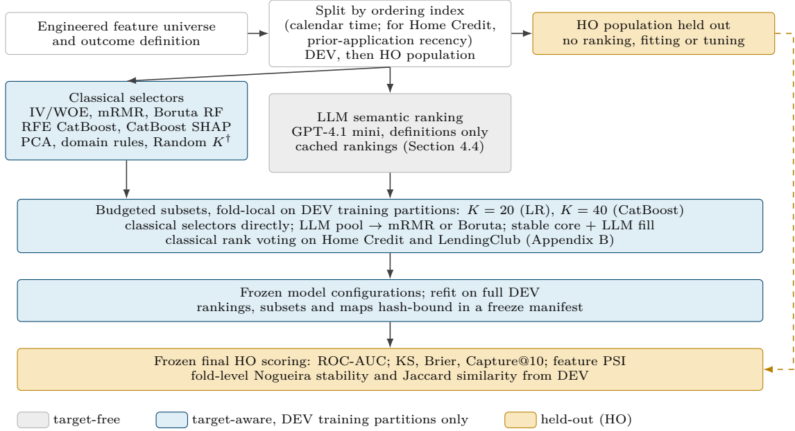
Figure 1: Research pipeline. Grey boxes are target-free stages that consume metadata only; blue boxes are target-aware stages confined to DEV training partitions and refitted once on full DEV, except that PCA, domain rules and Random K ( \dagger ), grouped with the classical selectors, are themselves target-free (Table 1); orange boxes concern the held-out population (HO), which the frozen final pipelines score once; the HO populations were inspected in earlier protocol versions (Section 4.6), so this is a frozen final scoring run, not a first look. The ordering index of the split is calendar time for LendingClub and Stability 2024 and prior-application recency for Home Credit.
