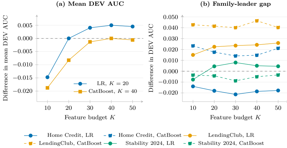
Figure C.1: Feature-budget sensitivity on development data. (a) Mean development AUC of all selectors of a backbone at each budget, measured against that backbone’s documented budget (logistic regression K = 20 , CatBoost K = 40 ; zero by construction at those points). (b) Development AUC of the LLM-assisted family leader minus that of the classical family leader, in each dataset–backbone case; positive values favour LLM-assisted selection. Circles and solid lines are logistic regression, squares and dashed lines CatBoost. No held-out observation enters either panel.
