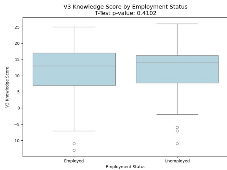
Box Plot
