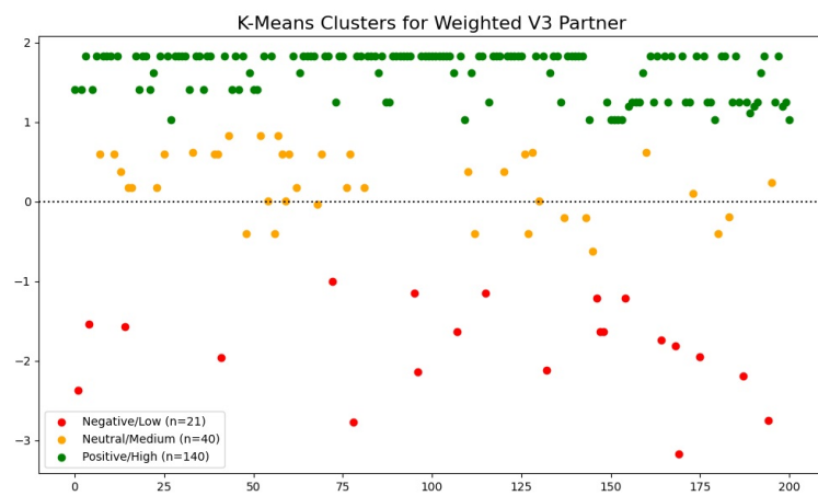
K-Means Clusters
