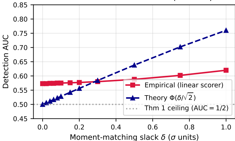
Theorem 1 Phase Transition (E1 + C1)
