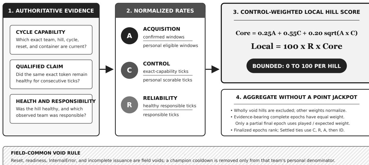
Figure 2. The checker admits current evidence; only immutable results enter epoch scoring.
