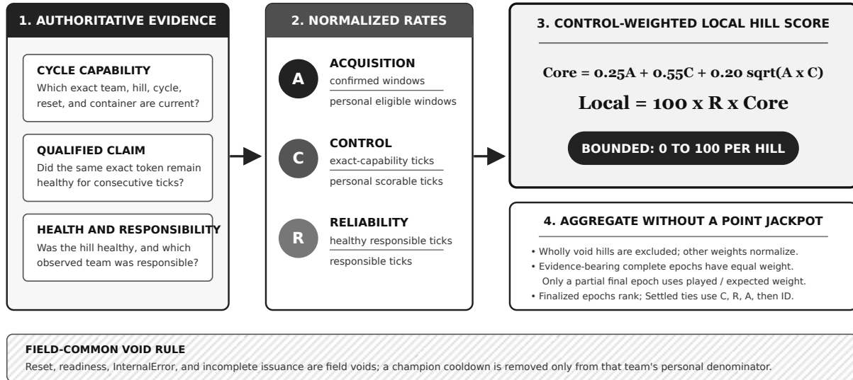
Figure 3. Formula version 2 pipeline. Exact cycle/container evidence becomes bounded personal rates before hill normalization and finalized-epoch aggregation.
