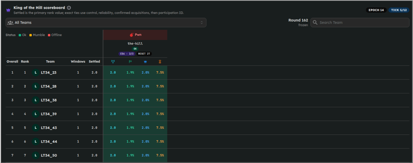
Figure 4. RSCTF formula version 2 scoring interface captured from the Docker Compose deployment on 14 July 2026 after the retained one-hour, 100-team event settled. The board shows ordinal ranks and the upper-right Epoch 14 and Tick 5/12 badges; the former cycle-length header badge is absent. The screen is application output, not a static mockup.
