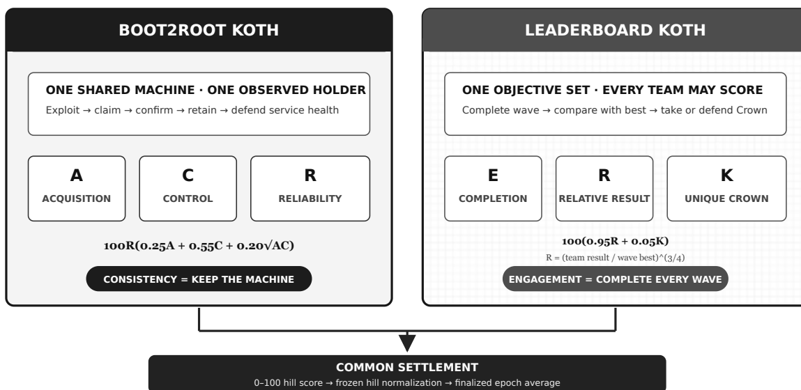
Figure 1. Boot2Root measures exclusive machine control. Leaderboard measures fresh, relative concurrent performance and one recurring per-wave Crown.
