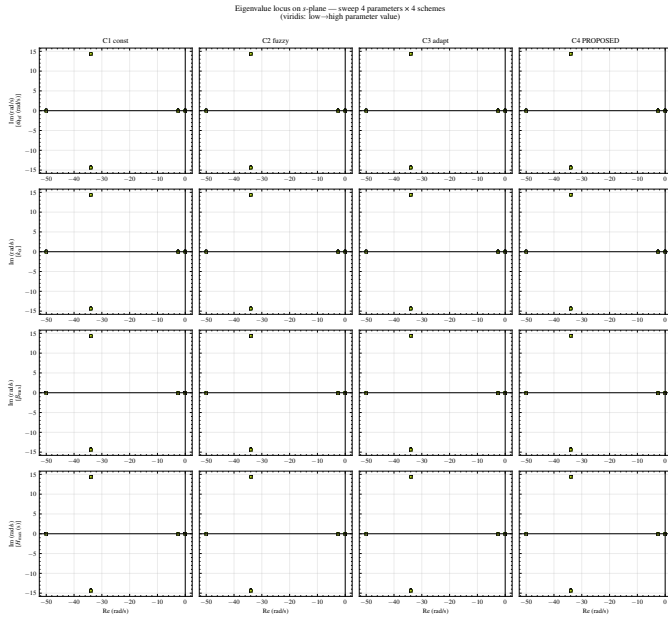
Fig. 5: Eigenvalue locus on the s -plane for sweeps of \omega_{\text{ref}} \in [0.5, 3] \text{ Hz/s} , k_\alpha \in [2, 10] , \beta_{\text{max}} \in [0.1, 1.0] , H_{\text{max}} \in [1, 8] \text{ s} (viridis: low \rightarrow high). All loci in the LHP.
