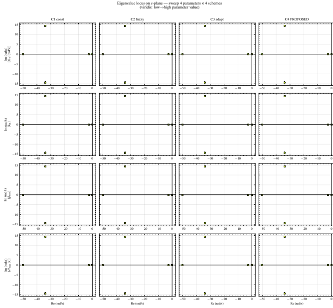
Fig. 5: Eigenvalue locus on the s -plane for sweeps of \omega_{\text{ref}} , k_\alpha , \beta_{\text{max}} , H_{\text{max}} (viridis: low→high). All loci in the LHP.
