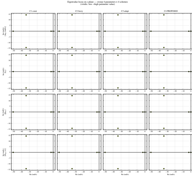
Fig. 5: Eigenvalue locus on the s -plane for sweeps of \dot{\omega}_{\text{ref}} , k_{\alpha} , \beta_{\text{max}} , H_{\text{max}} (viridis: low→high). All loci in the LHP.
