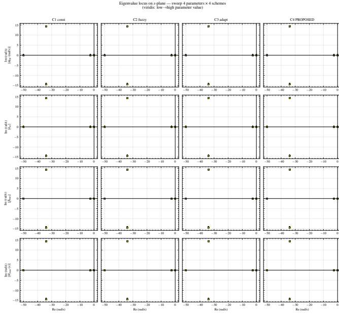
Fig. 5: Eigenvalue locus on the s -plane for sweeps of \omega_{\text{ref}} \in [0.5, 3] \text{ Hz/s} , k_\alpha \in [2, 10] , \beta_{\text{max}} \in [0.1, 1.0] , H_{\text{max}} \in [1, 8] \text{ s} (viridis: low \rightarrow high). All loci in the LHP.
