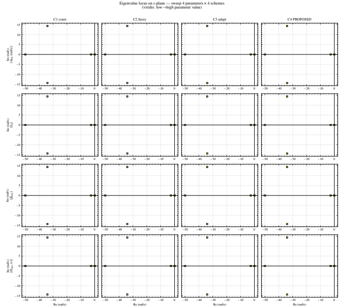
Fig. 4: Eigenvalue locus on the s -plane for sweeps of \omega_{\text{ref}} , k_{\alpha} , \beta_{\text{max}} , H_{\text{max}} (viridis: low→high). All loci in the LHP.
