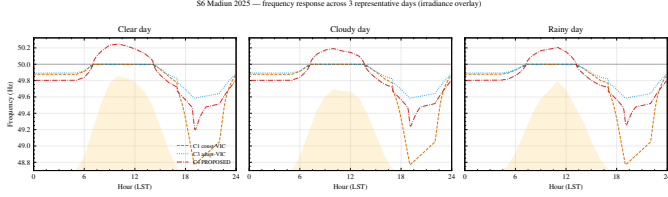
Fig. 6: Frequency response on three representative days (2025-08-01 clear, 2025-06-12 cloudy, 2025-10-25 rainy); irradiance overlaid (yellow). C0 omitted (diverges).
