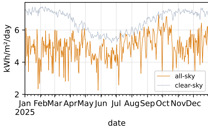
Daily irradiance --- Madiun 2025
