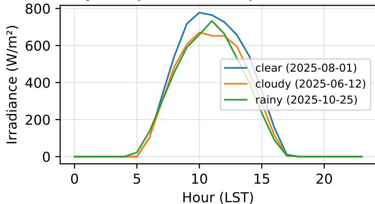
Hourly G(t) profile --- 3 representative days
