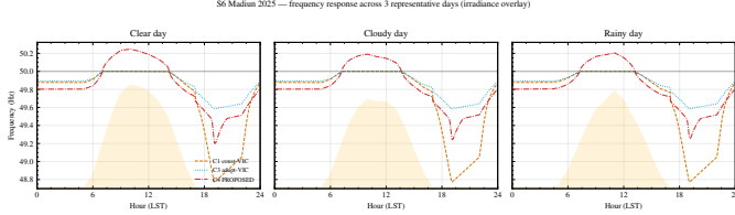
Fig. 6: Frequency response on three representative days (2025-08-01 clear, 2025-06-12 cloudy, 2025-10-25 rainy); irradiance overlaid (yellow). C0 omitted (diverges).
