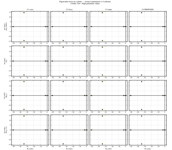
Fig. 4: Eigenvalue locus on the s -plane for sweeps of \omega_{\text{ref}} , k_{\alpha} , \beta_{\text{max}} , H_{\text{max}} (viridis: low \rightarrow high). All loci in the LHP.
