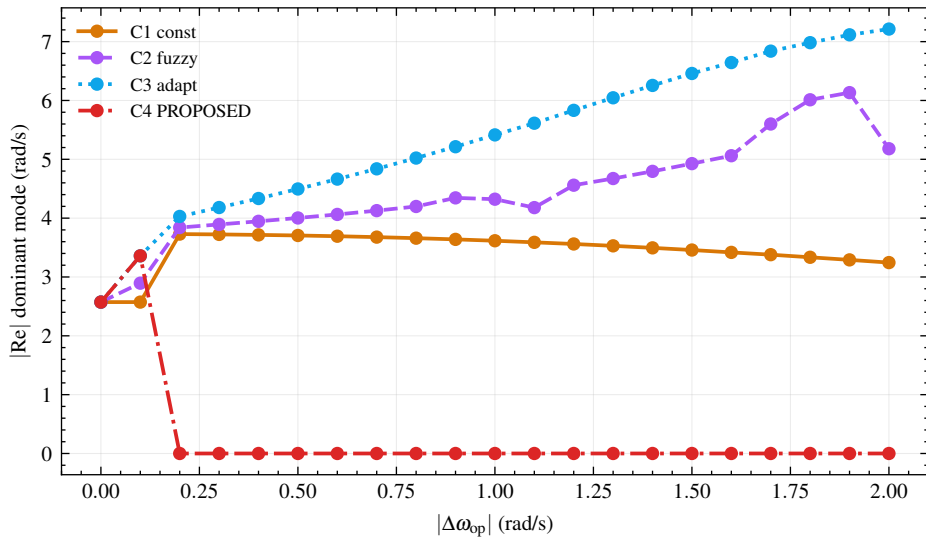
Dominant mode decay rate vs operating-point deviation
