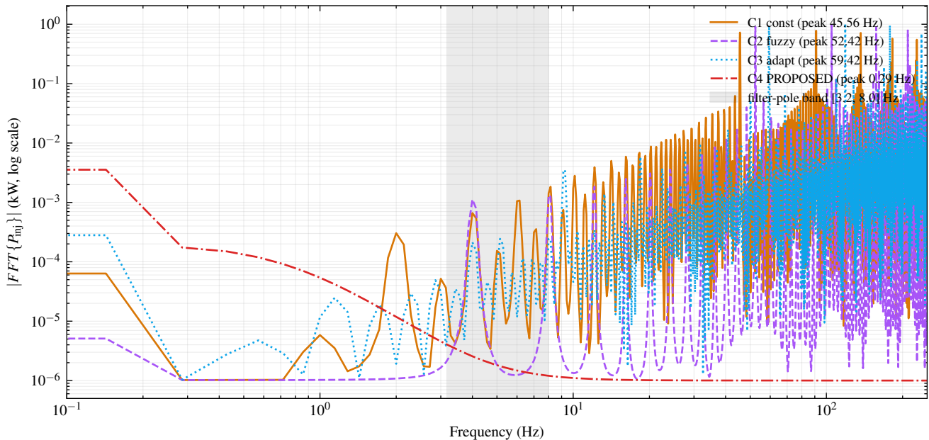
S1 steady-state spectrum — limit cycle frequency
