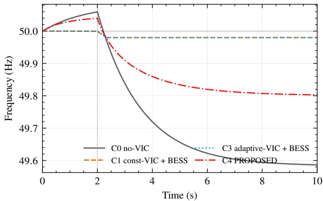
S1 — Load step +5% at t = 2 s, H_{\text{sys}} = 4 s, D_{\text{sys}} = 5
