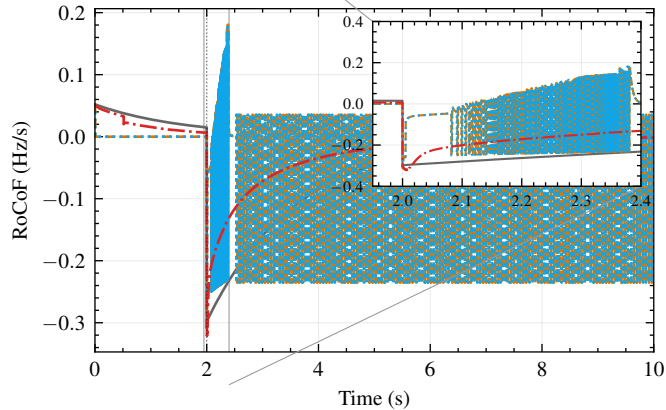
S1 — Load step +5% at t = 2 s, H_{\text{sys}} = 4 s, D_{\text{sys}} = 5
