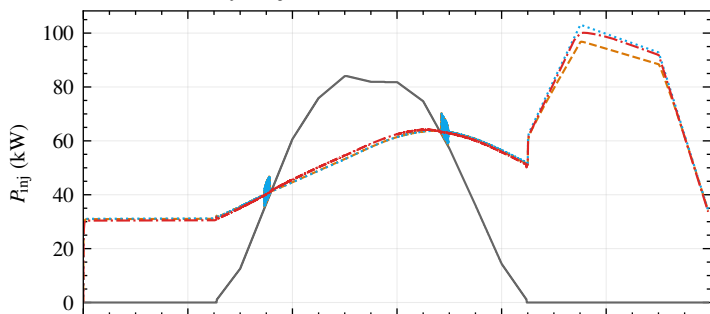
Daya BESS (positive = discharge)
