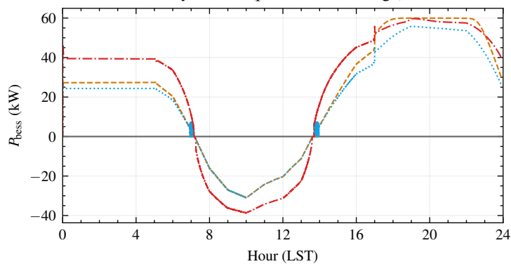
Daya BESS (positive = discharge)
