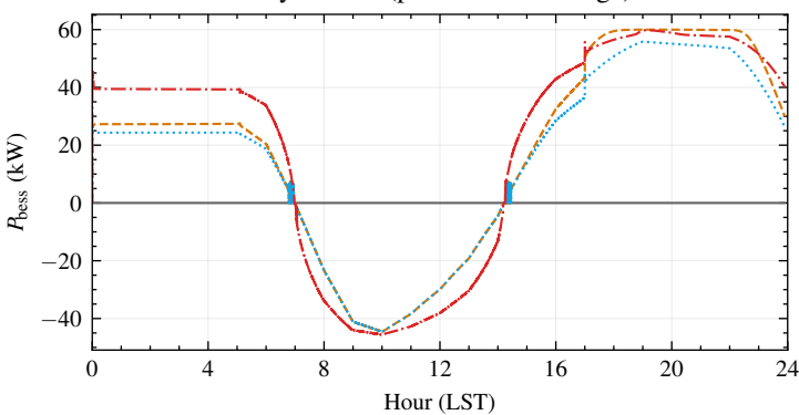
Daya BESS (positive = discharge)
