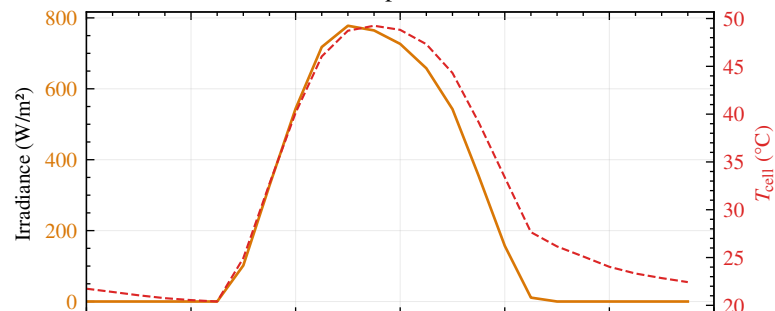
Irradiance and cell temperature — Madiun Clear
