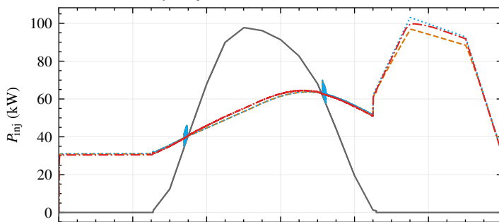
Daya injeksi total (PV + VIC + BESS)
