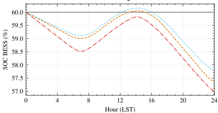
State-of-Charge BESS
