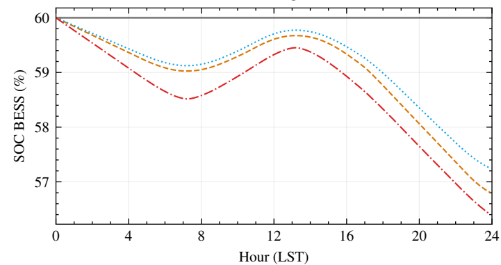
State-of-Charge BESS
