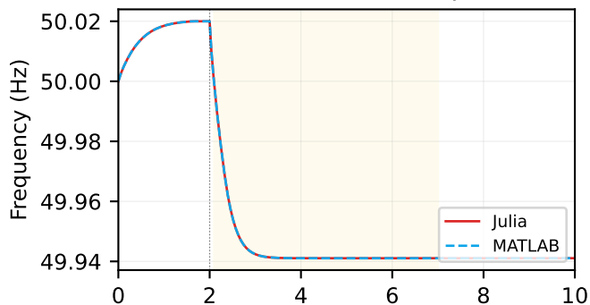
f(t) — RMSE = 1.60 \mu\text{Hz}
