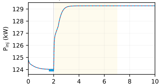
P_{\text{inj}} — RMSE = 0.060 W
