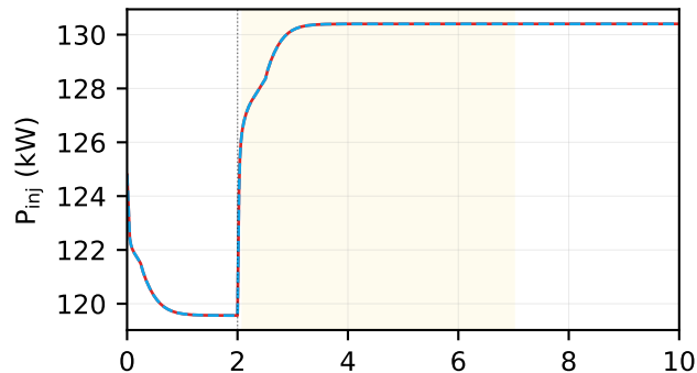
P_{\text{inj}} — RMSE = 0.001 W
