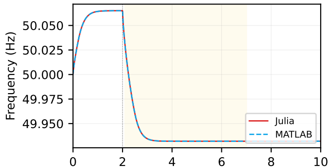
f(t) — RMSE = 0.05 \mu\text{Hz}
