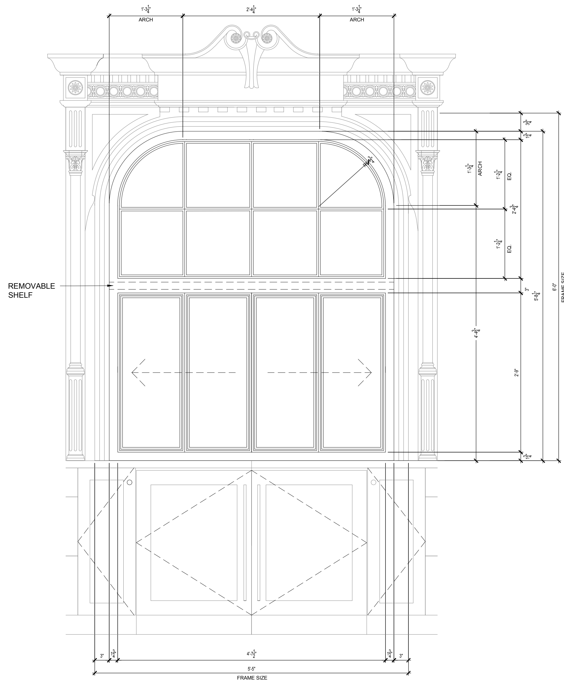
X BAR WINDOW - ENLARGED ELEVATION SCALE: 1" = 1'-0"
