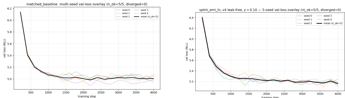
(a) matched_baseline (leak-immune by construction), 5 seeds, 0/5 diverged.
