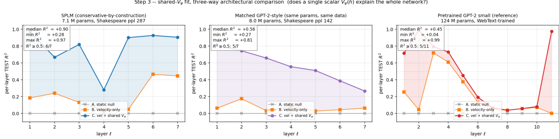
Figure 14: Shared- V_\psi per-layer TEST R^2 across three architectures on the same 50-sentence Tiny Shakespeare corpus. Left: SPLM ( d=128, L=8 , conservative-by-construction; 7.1 M parameters). Middle: Matched GPT-2-style decoder ( d=128, L=8, n_{\text{head}}=4 ; 8.0 M parameters; trained identically on the same corpus, better LM by val perplexity 142 vs. 287). Right: Pretrained GPT-2 small ( d=768, L=12 ; 124 M parameters). Three qualitatively distinct shapes (uniform / monotonic decay / bathtub) emerge from an identical diagnostic; the figure is the paper’s headline shared-potential separator.
