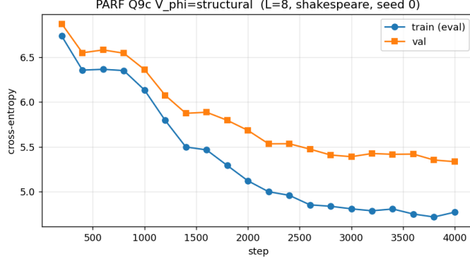
Figure 33: P1.6 wider structural V_\phi ( \phi/\theta=128 ), seed 0, val PPL 207.58 . The \sim 7\times widening of the internal §5.1 MLPs leaves the train-loss floor and val PPL essentially unchanged from P1, localising the binding constraint of Algorithm A in the dense regime to the O(BT^2) aggregation under the test-particle reduction (Theorem 60) rather than to V_\phi width.
