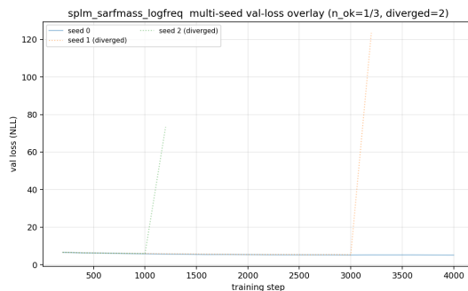
(c) splm_sarfmass_logfreq (no LN), 3 seeds, 2/3 diverged (dotted). The divergence-rate observation is the architectural content of this panel.
