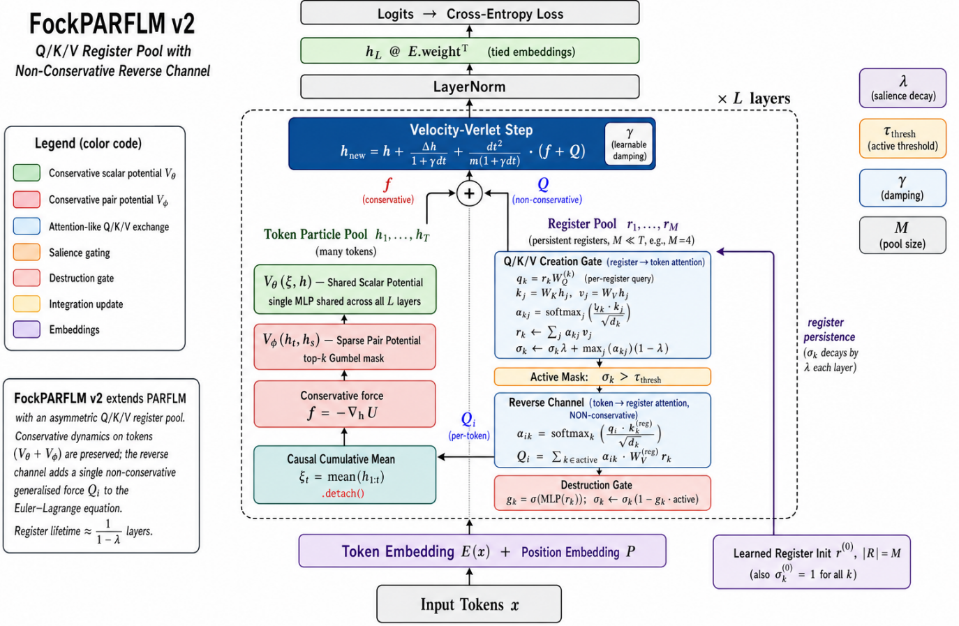
Figure 31: Architecture of FockPARFLM v2 — the Q/K/V register pool with non-conservative reverse channel. The model extends PARFLM (Figure 30) with a small persistent pool of M register particles r_1, \dots, r_M (right column) that exchange information with the T token particles h_1, \dots, h_T (left column) through two asymmetric attention-like pathways at every layer. The Q/K/V Creation Gate (light-blue, register \rightarrow token) lets each register attend over the input tokens (Equation (136)–Equation (139)), updating both its content r_k and its saliency \sigma_k under exponential decay \lambda ; an active mask \sigma_k > \tau_{\text{thresh}} then gates which registers participate downstream. The Reverse Channel (light-blue, token \rightarrow register) lets each token read from active registers, producing a per-token non-conservative generalised force Q_i (Equation (140)) that is summed with the conservative PARF force f = -\nabla_h U (where U = V_\theta + V_\phi ) before the damped Velocity-Verlet step. A per-register Destruction Gate (salmon) decays saliency to model annihilation a_v|\psi\rangle . The register state (r_k, \sigma_k) persists across layers with characteristic lifetime \tau_{\text{life}} \approx 1/(1-\lambda) (loop on the right margin), providing cross-layer working memory that token-token attention lacks. Only the reverse channel breaks conservativity; V_\theta and V_\phi remain Helmholtz-conservative scalar potentials shared across all L layers, so the shared-potential R^2 separator of Section 15 remains diagnostic. Source: notebooks/conservative_arch/parf/model_fock_parf_v2.py.
