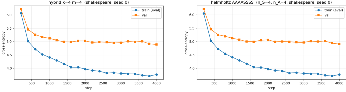
(a) Variant A ( k=4, m=4 ) seed 0, val PPL 133.01 .
