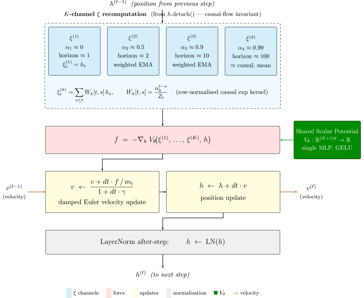
Figure 10: Detail of a single multi-channel SPLM integration step (one of the L steps in the SPLM Stage of Figure 9). Row 1 (cyan): the K -channel context summary \xi^{(k)} is recomputed from h.detach() via a row-normalised causal exponential kernel with per-channel decay \alpha_k , spanning effective horizons from \sim 1 to \sim 100 tokens. Row 2 (red): the conservative force f = -\nabla_h V_\theta(\xi^{(1)}, \dots, \xi^{(K)}, h) is computed from the shared scalar potential V_\theta (green). Row 3 (yellow): a damped Euler velocity update with per-token logfreq mass m_t and learnable damping \gamma , followed by a position update. Row 4 (gray): LayerNorm is applied after each step. Orange arrows show velocity threading across steps; the shared V_\theta is the same single-MLP network at every step and for all K channels.
