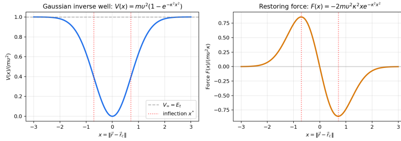
Figure 1: The Gaussian semantic energy well V(x) = \mathfrak{m}v^2(1 - e^{-\kappa^2 x^2}) . The potential is flat at the centroid (no net force on a well-placed particle), steepest at x^* = 1/(\kappa\sqrt{2}) , and saturates at the total ensemble energy E_t = \mathfrak{m}v^2 . Beyond the inflection point, the restoring force decreases rapidly — a particle that strays far from the ensemble is effectively free, modulo interactions with other ensembles.
