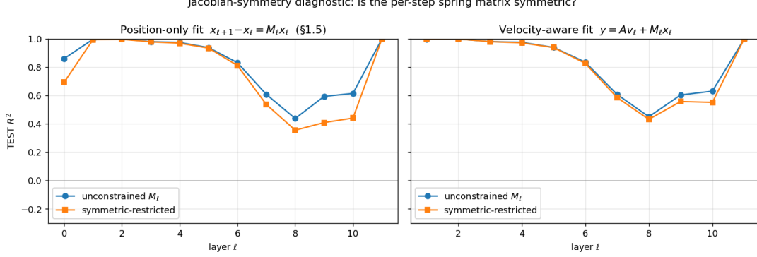
Figure 13: Velocity-aware Jacobian-symmetry diagnostic on PCA-16, pretrained GPT-2 small (panel 3 of 3). The symmetric-restricted fit tracks the unconstrained fit within \leq 0.08 at every layer, so the pretrained model also passes Q-loc once the velocity-term confound is removed. The literature §1.5 reading of GPT-2 as harbouring a large non-conservative (skew / curl) component was an artefact of the diagnostic; the per-step operators are symmetric.
