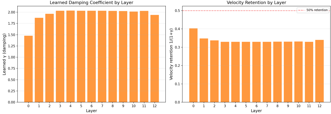
Figure 39: Learned damping coefficient \gamma (left) and velocity retention 1/(1+\gamma) (right) of the second-order model M2 at each GPT-2 layer. Layer 0 has the lowest damping ( \gamma = 1.48 , 40% velocity retention); all transformer layers saturate at \gamma \approx 2.0 (33% retention), deep in the overdamped regime. Even at the layer most favourable to second-order dynamics, the optimiser drives the model toward first-order behaviour.
