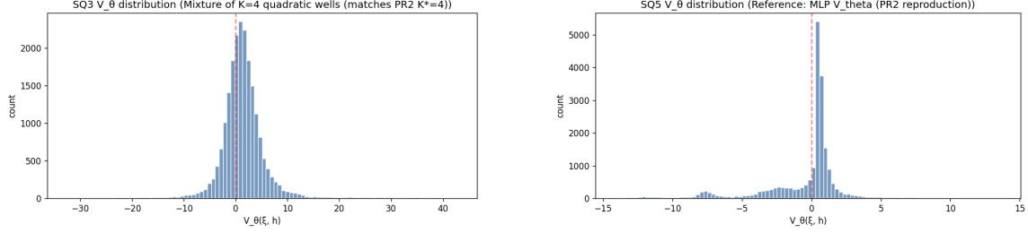
Figure 34: V_\theta distributions on real PARFLM trajectories. Left : SQ3 mixture-of- K=4 structured V_\theta (best PPL 184.5, range 75.4, std 3.90). Right : SQ5 unmodified MLP V_\theta reference (best PPL 221.4, range 27.8, std 2.73). SQ3 carries a heavier-tailed distribution but the bulk is narrower and centred; the MLP develops a bimodal shape with a negative side-lobe that signals initialisation instability. See Section B.9 for the FLOP analysis.
