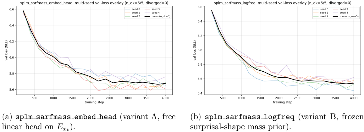
Figure 20: v4 leak-free S = 5 per-seed validation-loss overlays for the two per-token-mass arms of Section 15.17. The 1.31 – 1.59\times asymmetric inflation is visible directly: both variants now plateau in the 250–295 PPL range under causal honesty rather than the 160–223 PPL range of the v2 single-seed runs.
