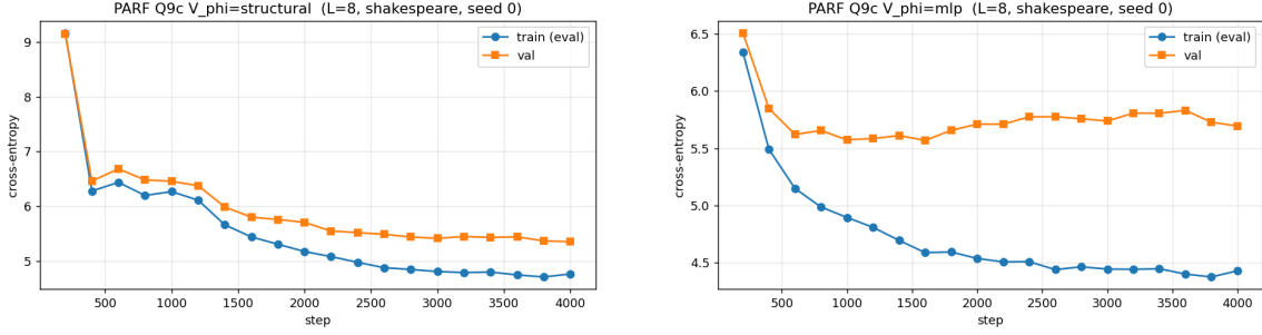
(a) Structural V_\phi (Equation (131)) seed 0, val PPL 210.5 . V_\phi params \sim 4,000 . (b) Unstructured MLP V_\phi (mlp_hidden = 16) seed 0, val PPL 297.2 . V_\phi params \sim 6,449 .
