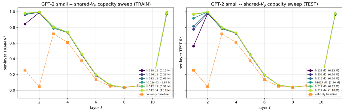
(b) Per-layer R^2 curves overlaid across the six capacities, shown for both TRAIN (left) and TEST (right) splits; visibly indistinguishable on the middle-layer plateau.
