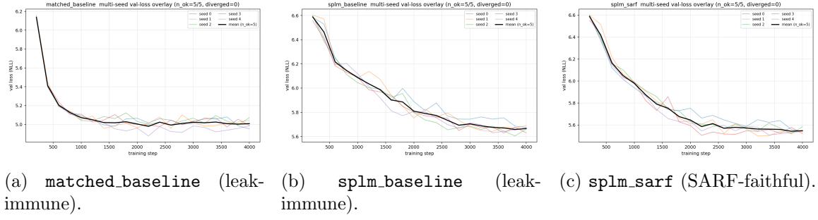
Figure 19: v4 leak-free S = 5 per-seed validation-loss overlays for the leak-immune controls and the SARF-faithful arm of Section 15.16. The two leak-immune cells reproduce their v2 means at 1.00\times ; the SARF-faithful arm inflates to 1.34\times under causal honesty.
