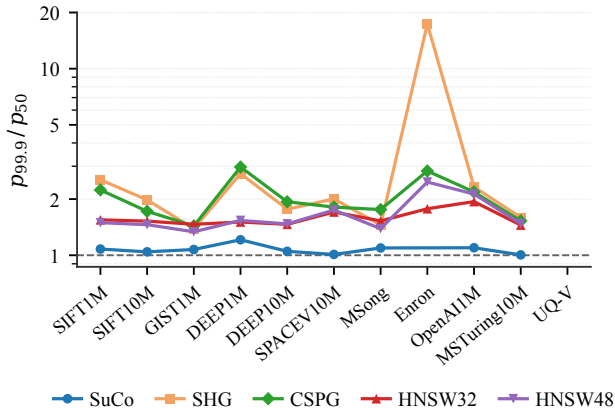
Tail-to-median latency at Recall@10 \geq 0.95
