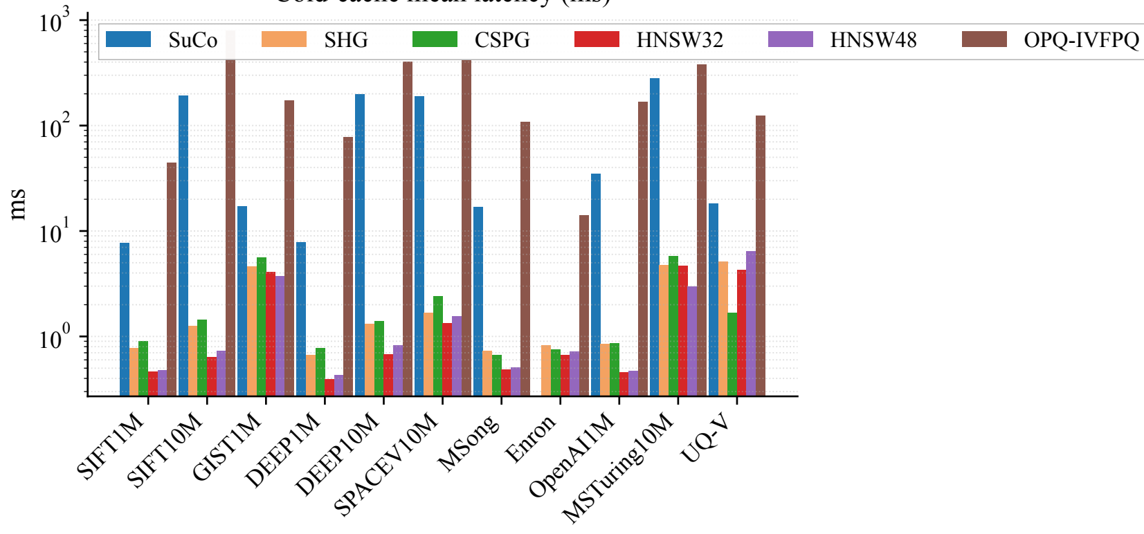
Cold-cache mean latency (ms)
