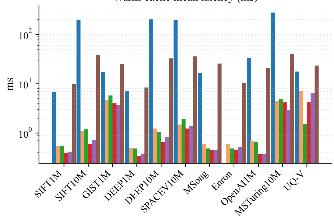
Warm-cache mean latency (ms)
