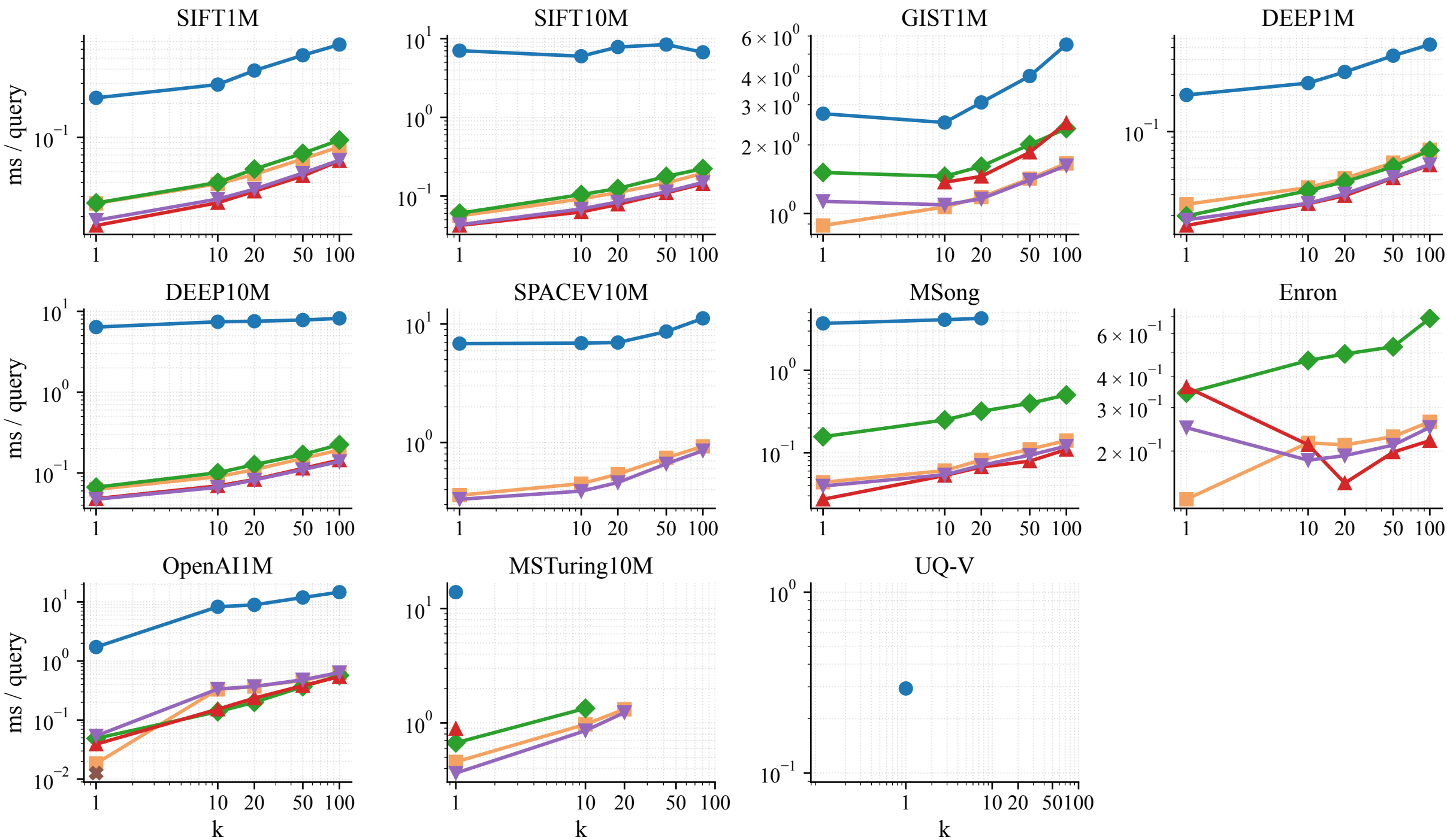
k sensitivity: ms/query at recall \geq 0.99
