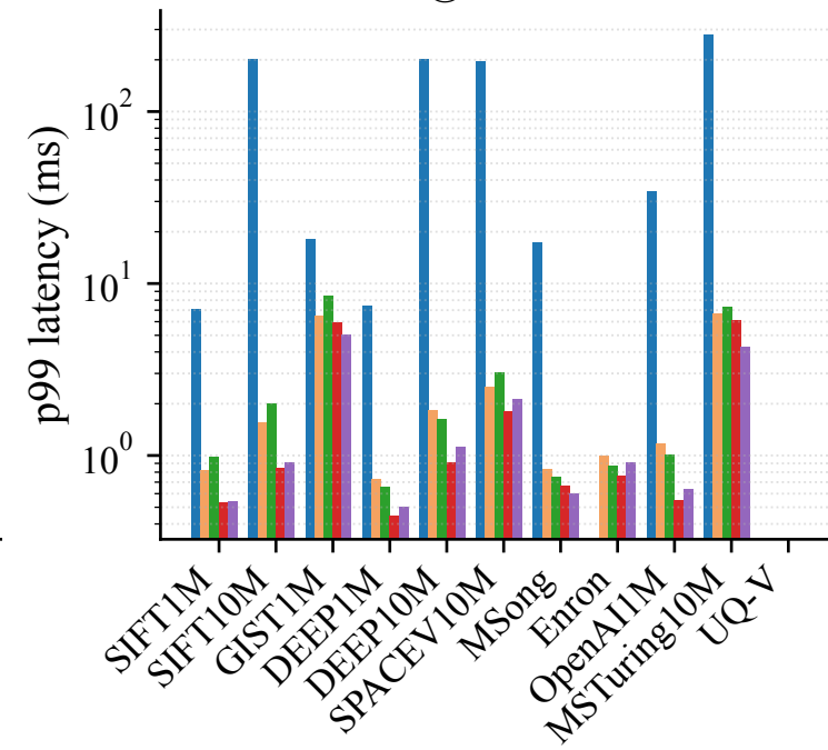
P99 @ recall 0.95
