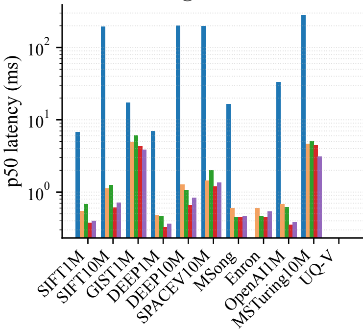
P50 @ recall 0.95
