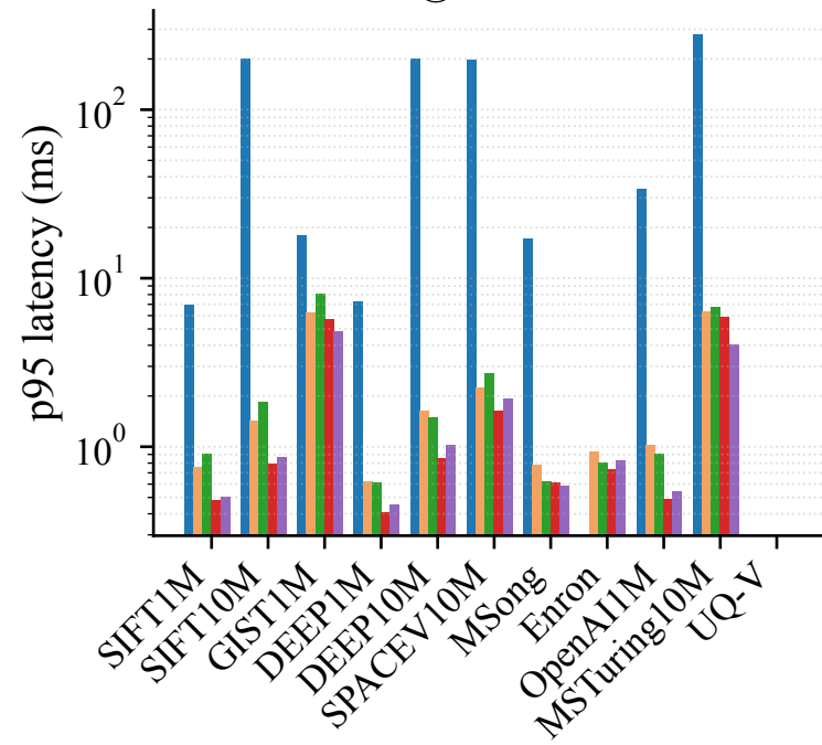
P95 @ recall 0.95
