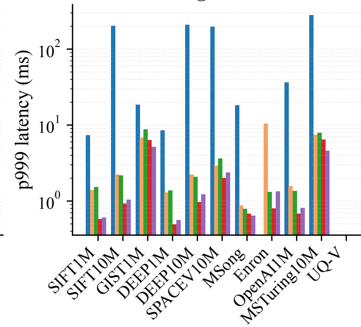
P999 @ recall 0.95
