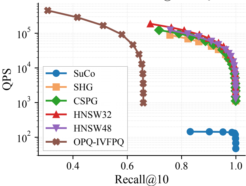
DEEP10M — Recall@10 vs QPS
