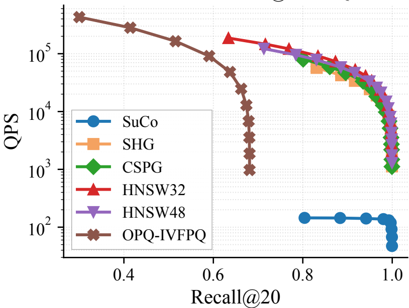
DEEP10M — Recall@20 vs QPS
