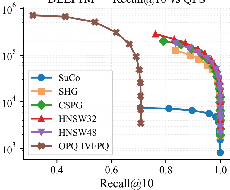
DEEP1M — Recall@10 vs QPS
