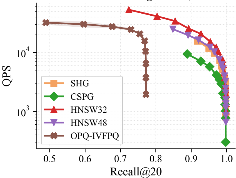
Enron — Recall@20 vs QPS
