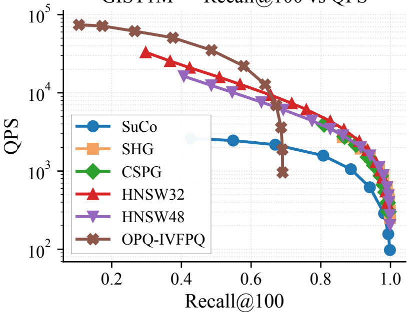
GIST1M — Recall@100 vs QPS
