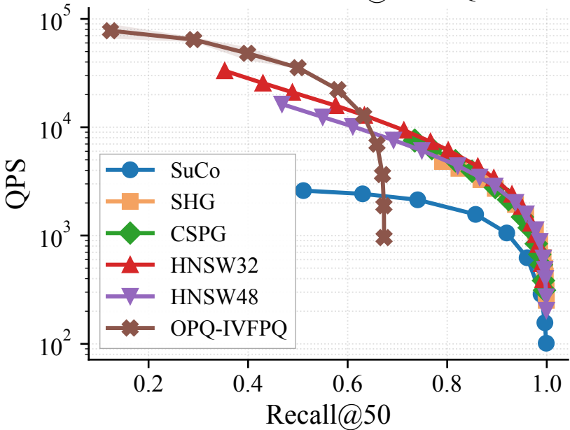
GIST1M — Recall@50 vs QPS
