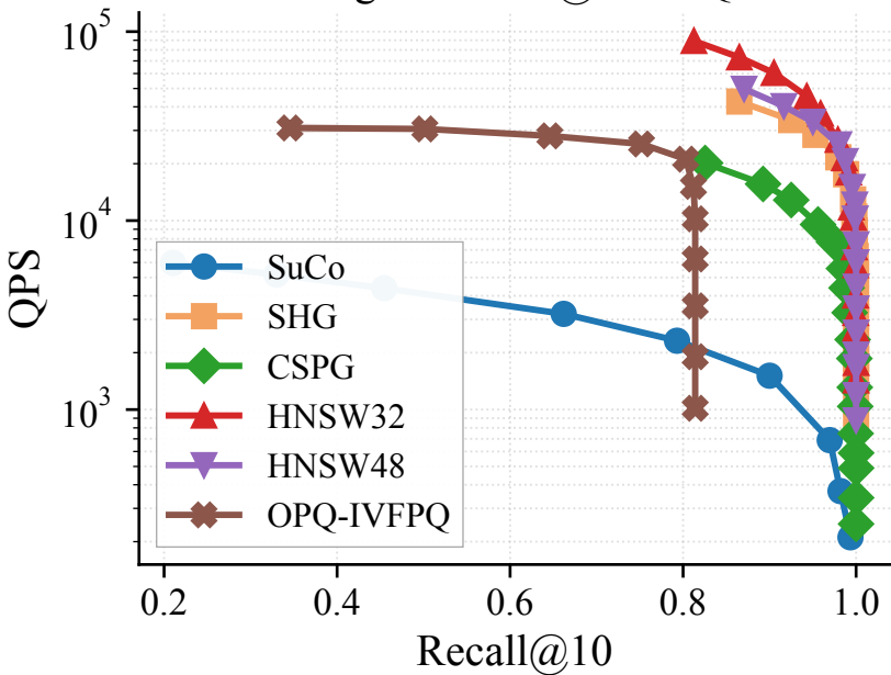
MSong — Recall@10 vs QPS
