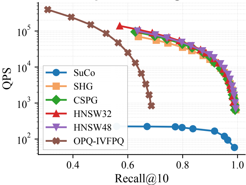
MSTuring10M — Recall@10 vs QPS
