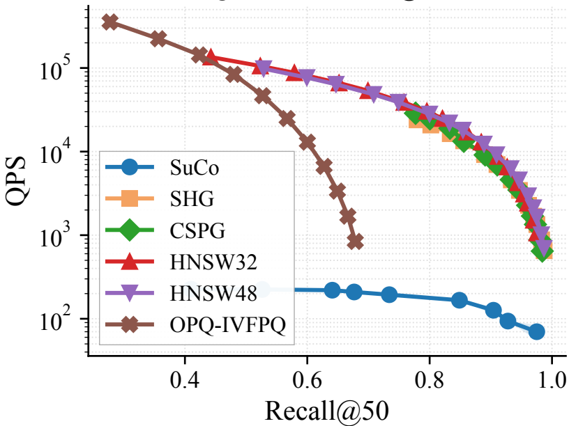
MSTuring10M — Recall@50 vs QPS
